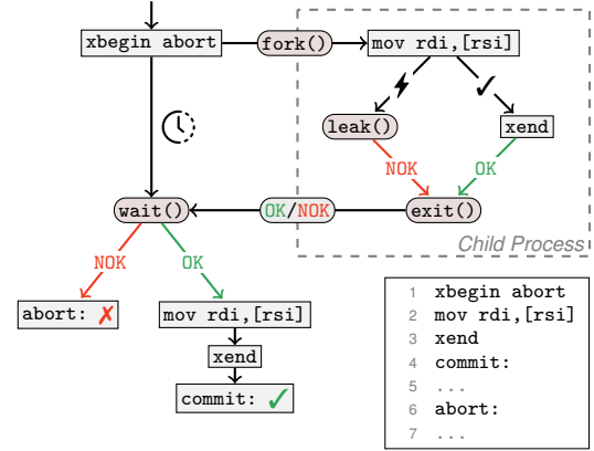
Figure 3: An illustration of Crucible’s TSX emulation on a simple code example. Crucible first executes the transaction in a child process, simulating leakage when encountering faults. Based on whether the child transaction succeeds, it then aborts (NOK) or commits (OK) the transaction in the parent process.
