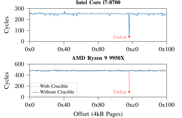
Figure 4: Access timings for buffer indexed with leaked kernel byte 0xba ( n=2000 ). Native leakage on Meltdown-affected CPU (top) is successfully replicated by Crucible on unaffected CPU (bottom).
