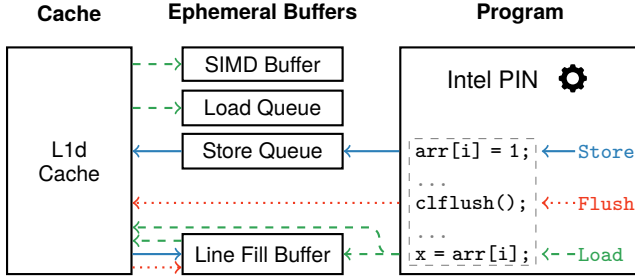
Figure 2: High-level illustration of Pin’s interaction with our default buffer model. Victim programs can trigger a store (solid line), load (dashed line), or flush (dotted line) path. The arrows indicate which buffers are affected by a specific path, and in which order. The load path may skip the line-fill buffer in case of an L1d hit.
